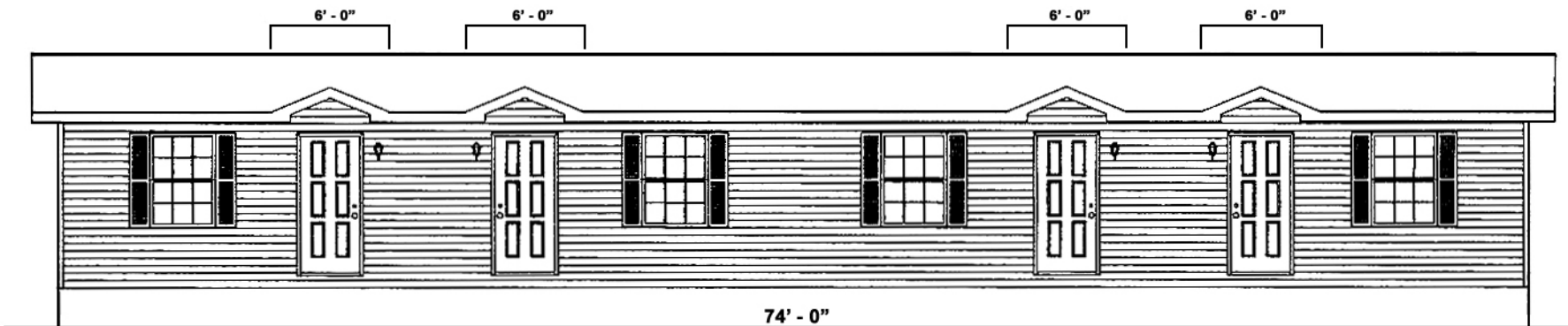
FRONT ELEVATION
